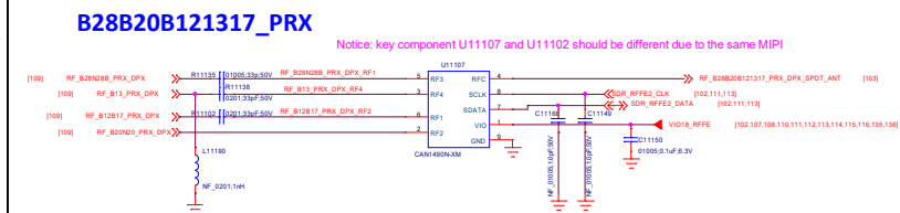
B28B20B121317_PRX
